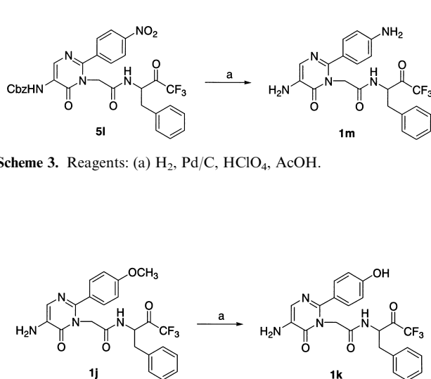
Scheme 4. Reagents: (a) \text{BBr}_3 , \text{CH}_2\text{Cl}_2 .
